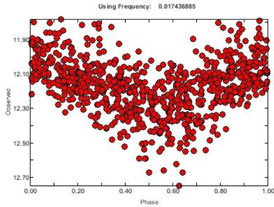
GSC 9449-00903 / 2MASS J18353947-7722296 / ASAS 183539-7722.4 – folded lightcurve ( P=57\pm 1d )
