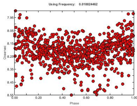
2MASS J02460684-6853254 / ASAS 024607-6853.4 – folded lightcurve ( P=53\pm 1.5d )
