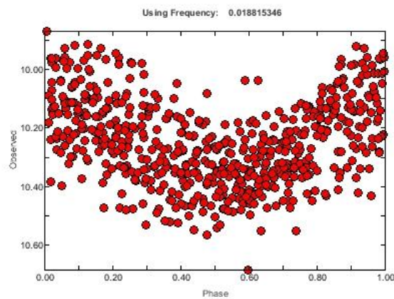
GSC 5497-00984 / 2MASS J10320280-1458556 / ASAS 103203-1458.9 – folded lightcurve ( P=53\pm 0.5d )
