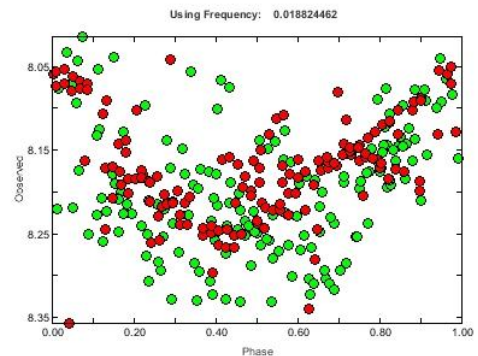
(4) HJD 2452056 - HJD 2452261 (red) HJD 2452447 - HJD 2453102 (green) folded with a period of 53.12d
