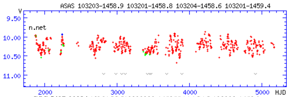
GSC 5497-00984 / 2MASS J10320280-1458556 / ASAS 103203-1458.9
