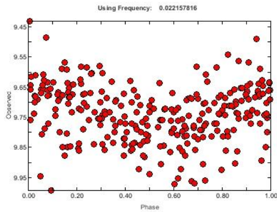
GSC 0595-01102 / 2MASS J00202233+0734155 / ASAS 002022+0734.3 – folded lightcurve (P=45±1d)
