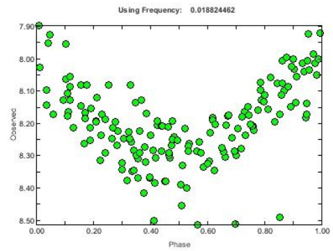
(2) HJD 2454320 - HJD 2454567 folded with a period of 53.12d
