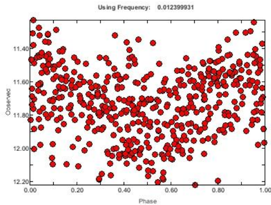
GSC 4704-00720 / 2MASS J02384781-0526508 / ASAS 023848-0526.8 – folded lightcurve (P=81±4d)
